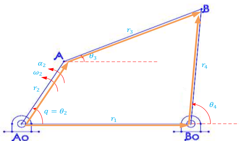
Figure 1. Four-Bar Mechanism
