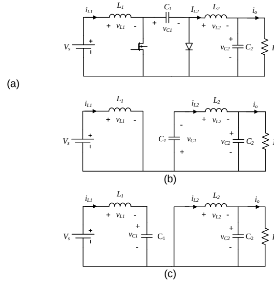
Fig. 2 Circuit diagrams of the Cuk converter. (a) actual circuit. (b) equivalent circuit in ON mode.
