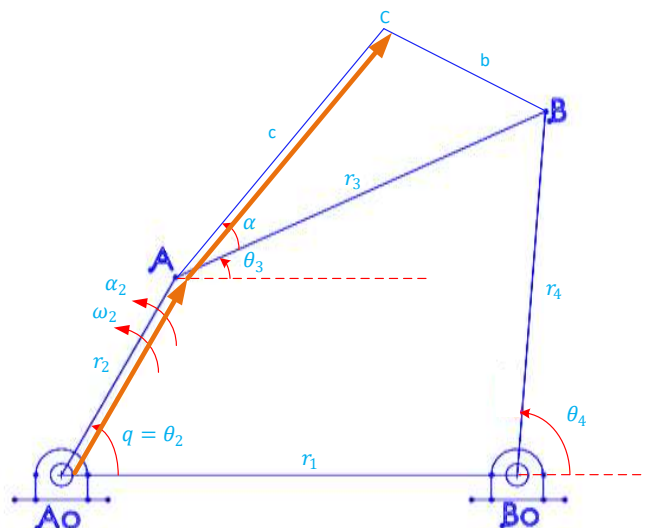
Figure 1. Four-Bar Mechanism
