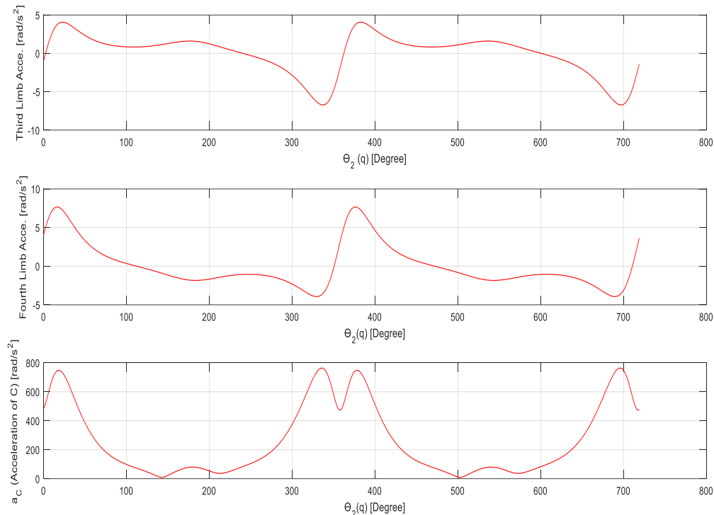
Figure 4. Limb and Point C Accelerations of Four-Bar Mechanism
