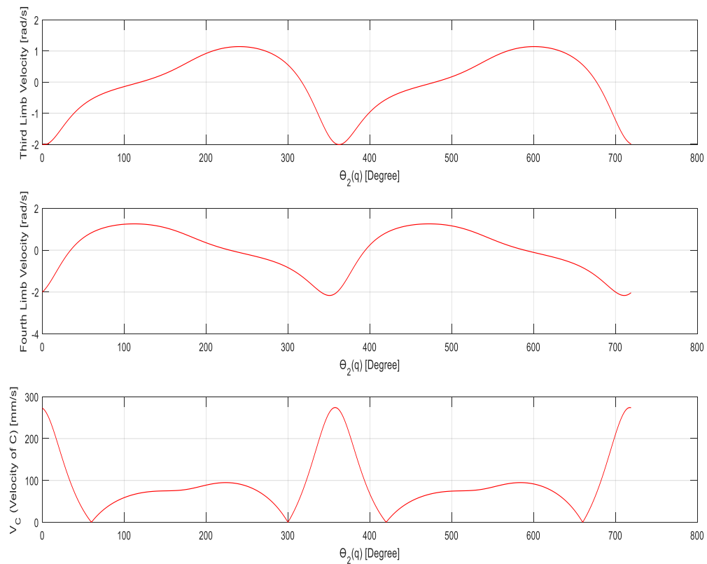
Figure 3. Limb and Point C Velocities of Four-Bar Mechanism
