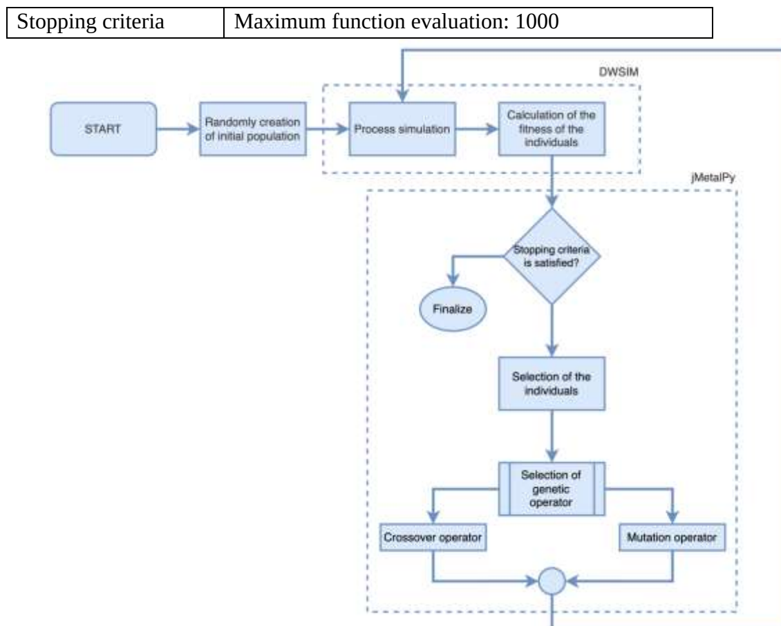
Figure 6. Integration of optimization method into the process simulator
